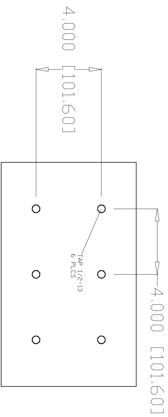
MOUNTING HOLE PATTERN
